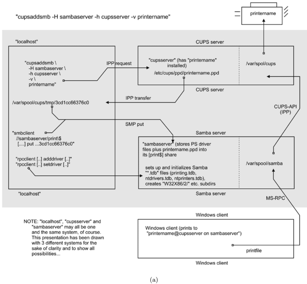
Figure 18.16. cupsaddsmb flowchart.
