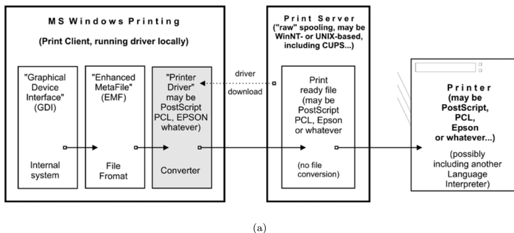
Figure 18.13. Print driver execution on the client.
