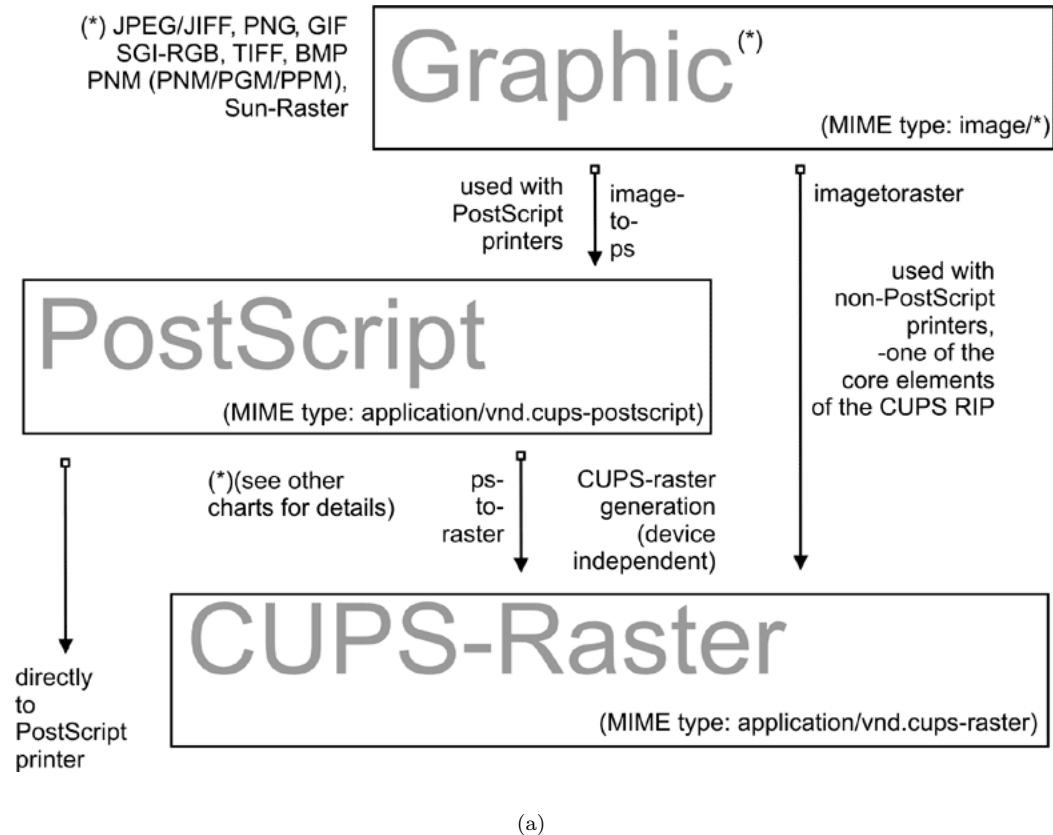
Figure 18.8. Image format to CUPS-raster format conversion.
