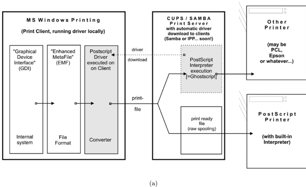
Figure 18.15. Printing via CUPS/Samba server.
