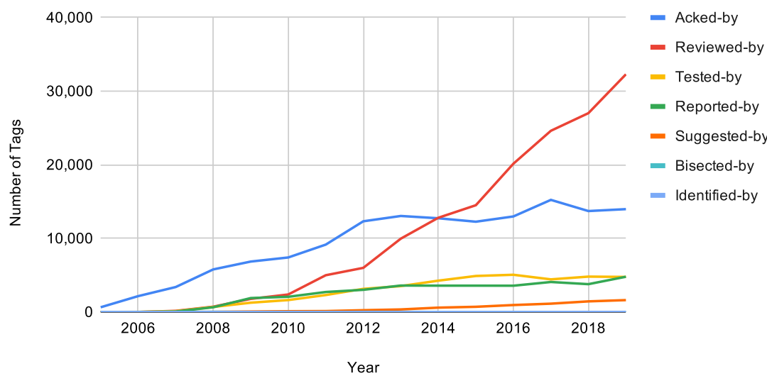
Tags in the Linux Kernel per Year (excluding signed-off-by)
