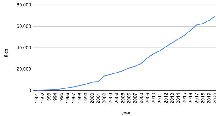
Number of Files in the Linux Kernel
