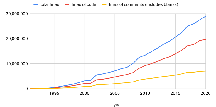
Lines of Code & Comments
